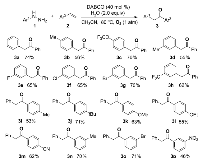
Scheme 2. Transition-metal-free selective synthesis of 1,2-diarylethane-1-one. For reaction Conditions, see Table 1, entry 6. Yields shown are of isolated products.
